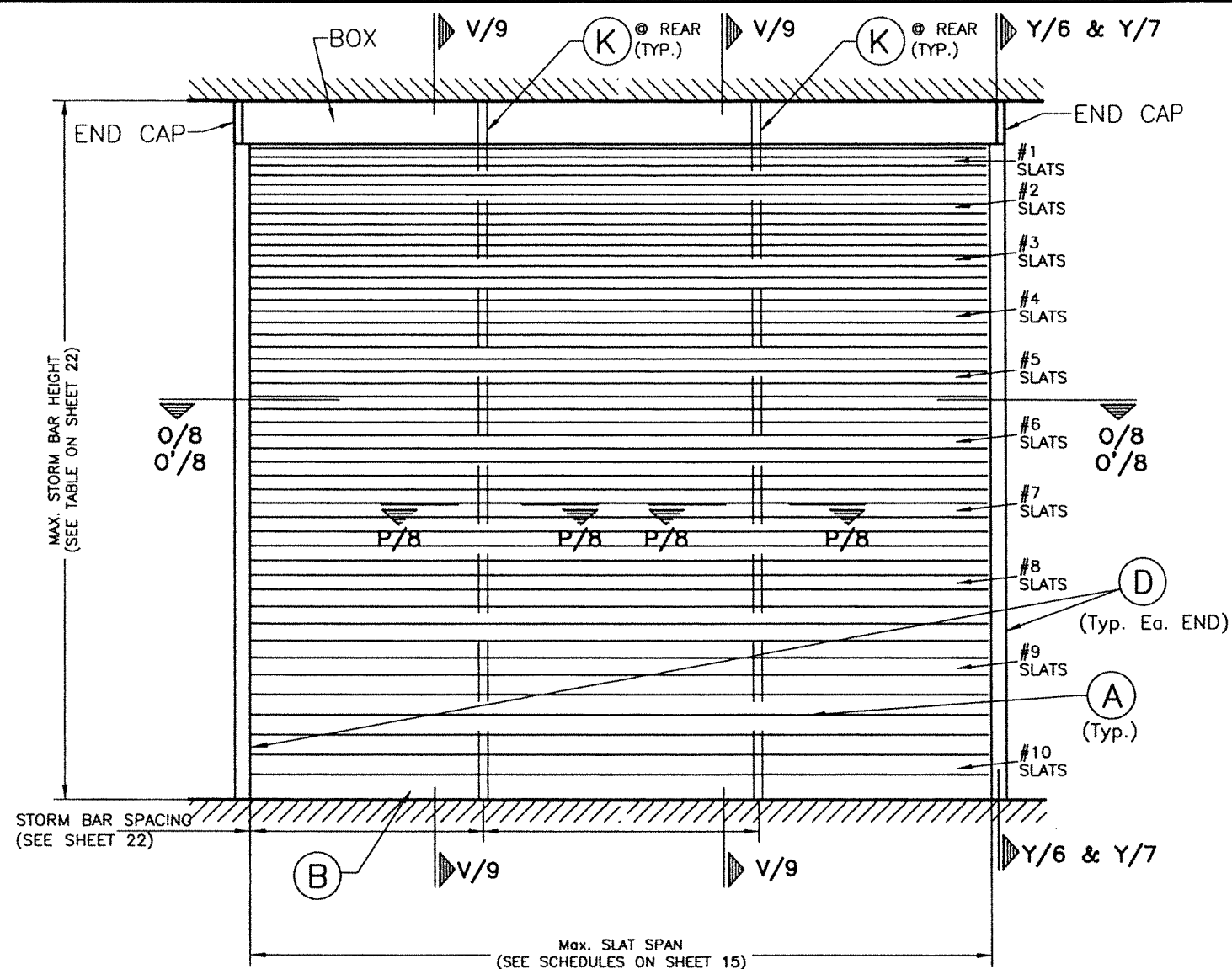
TYPICAL SINGLE UNIT ELEVATION W/ STORM BARS *
