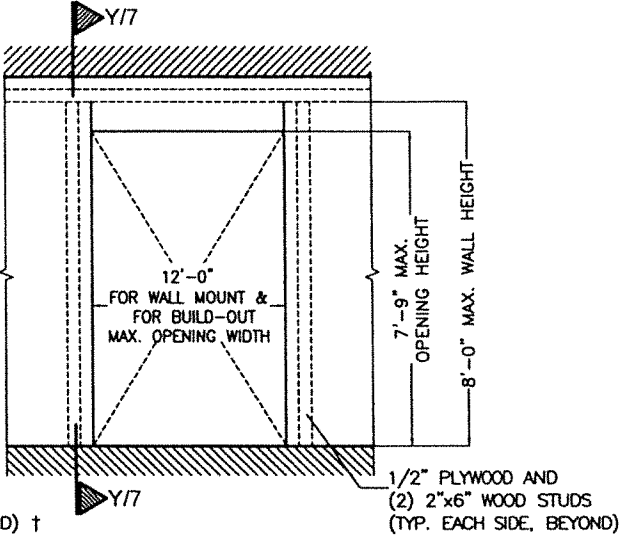
DETAIL 2 (ELEVATION)
