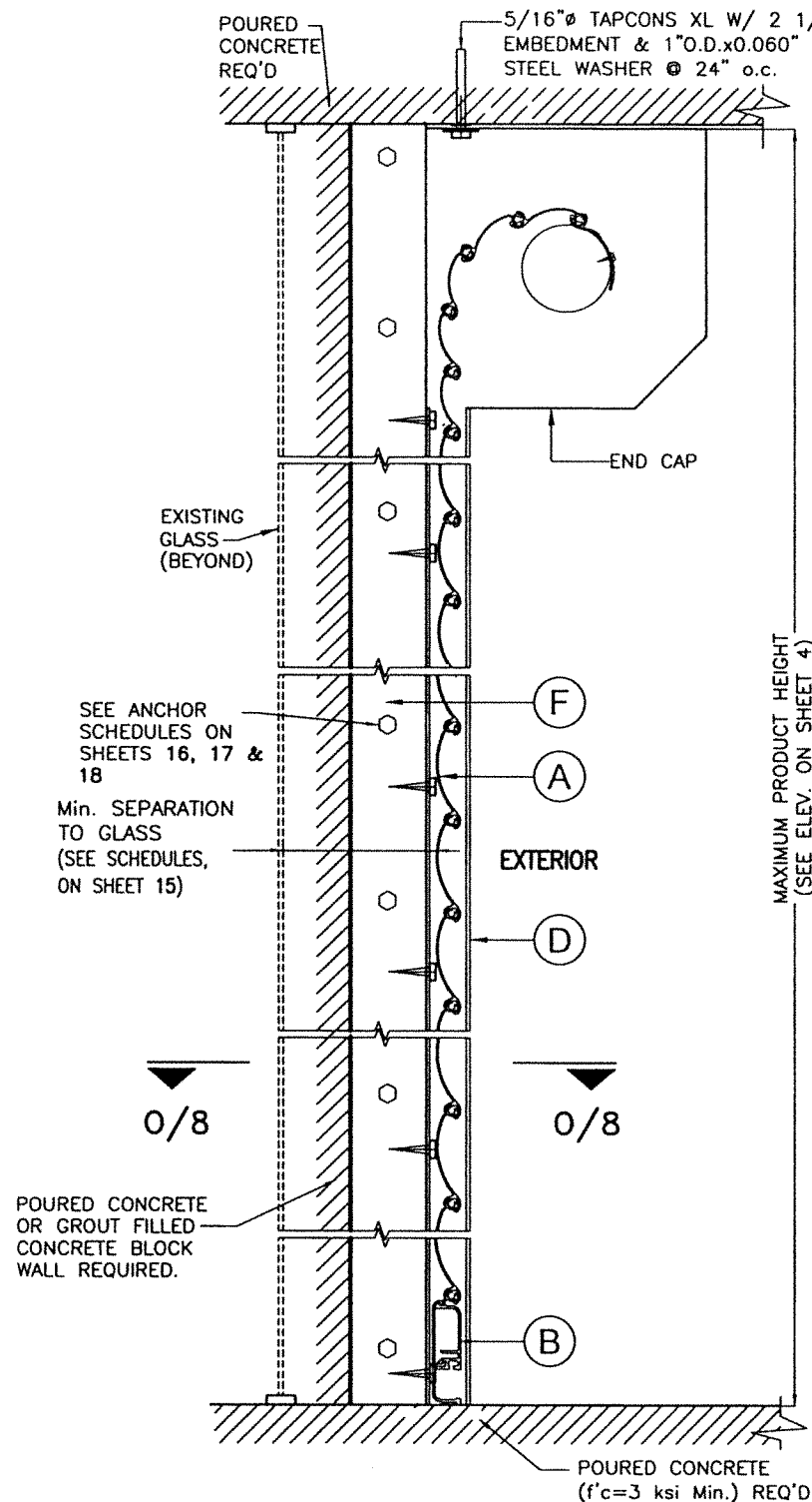
FLOOR/CEILING / TRAPPED MOUNTING *
