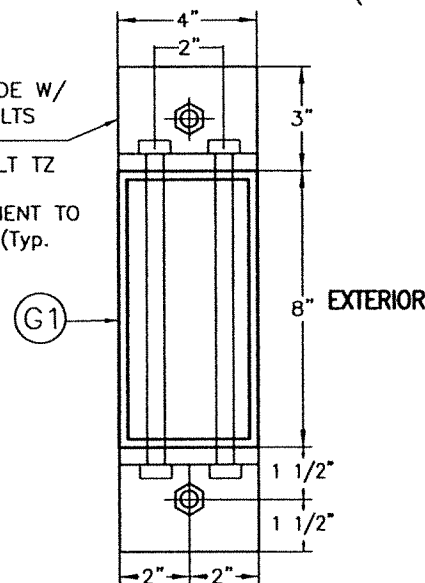
SECTION X1-X1 W/ (G1) * (END & INTERIOR MULLION) (W/ ORIENTATION # 1) (8"x4")
