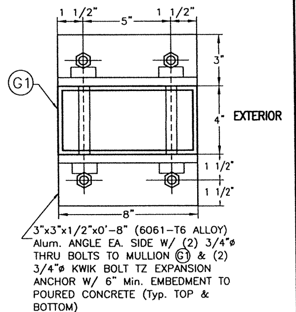
ALTERNATIVE SECTION X1-X1 W/ (G) * (END & INTERIOR MULLION) (W/ ORIENTATION # 2) (4"x6")
