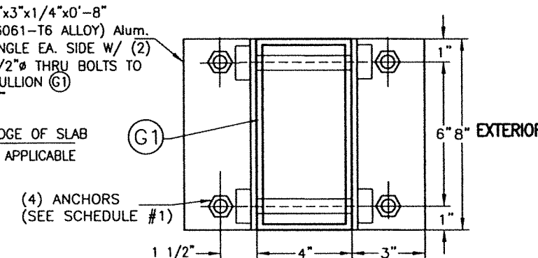
ALTERNATIVE SECTION X1-X1 W/ (G1) (4"x8" INTERIOR AND END MULLION ONLY W/ ORIENTATION # 1)
