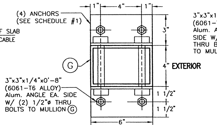
ALTERNATIVE SECTION X1-X1 W/ (G) (4"x6" INTERIOR MULLION ONLY W/ ORIENTATION # 2)
