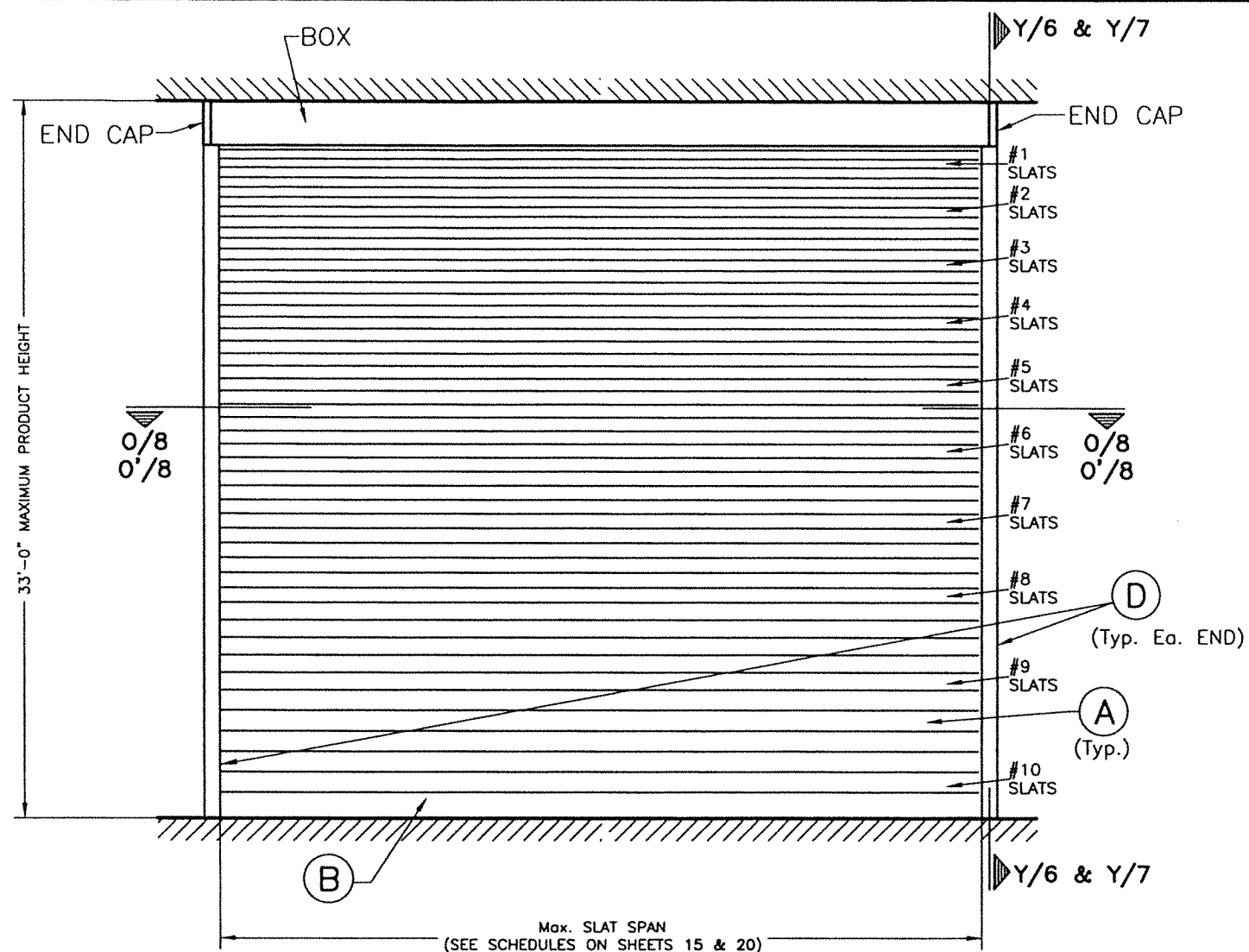
TYPICAL SINGLE UNIT ELEVATION W/O STORM BARS *, **
