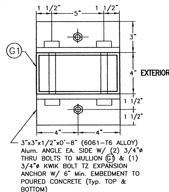
ALTERNATIVES SECTION X1-X1 W/ (G1) * (END MULLION ONLY) (W/ ORIENTATION # 2) (4"x8")
