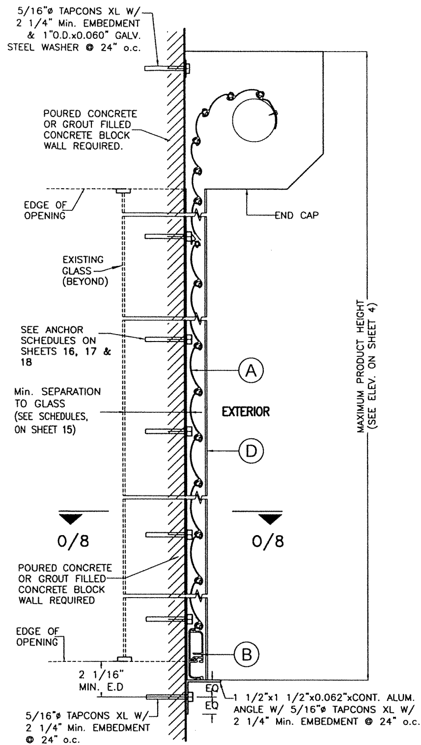
WALL MOUNTING *
