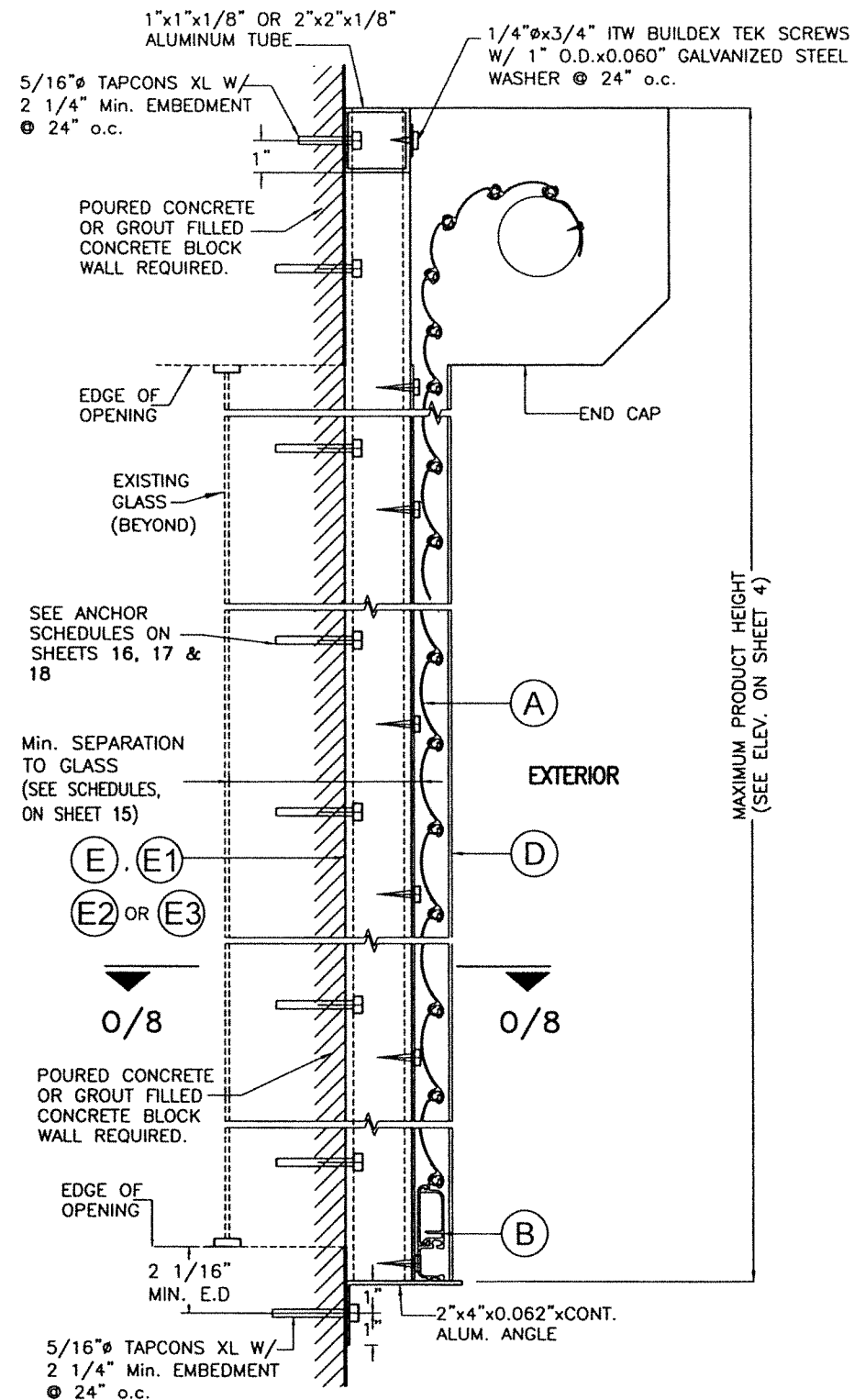
BUILD-OUT MOUNTING *
