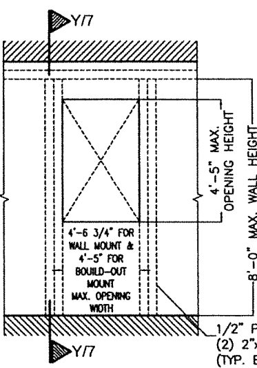
DETAIL 1 (ELEVATION)
