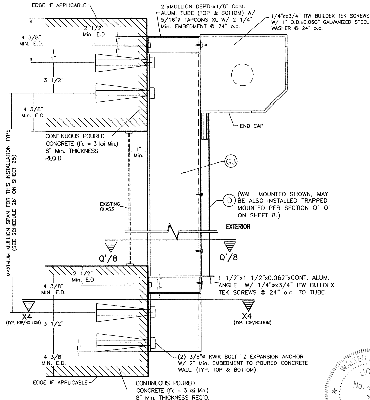
WALL MOUNTING: MULLION (G3) POURED CONCRETE WALL SECTION W-4
